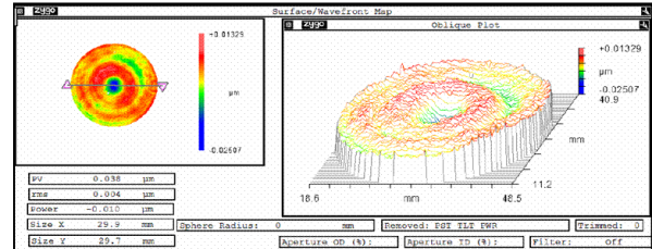
Form Accuracy: PV = 0.038 μm
