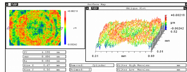
Surface Finish: Ra = 0.486 nm
