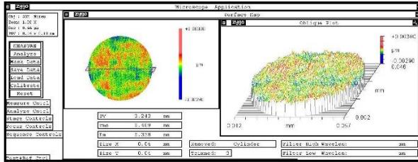
Surface Finish: Ra = 0.328 nm
