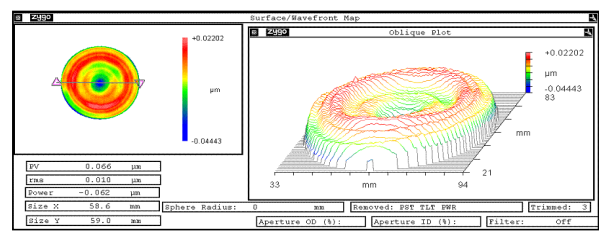
Form Accuracy: PV = 0.066 μm
