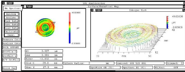
Form Accuracy: PV = 0.037 μm
